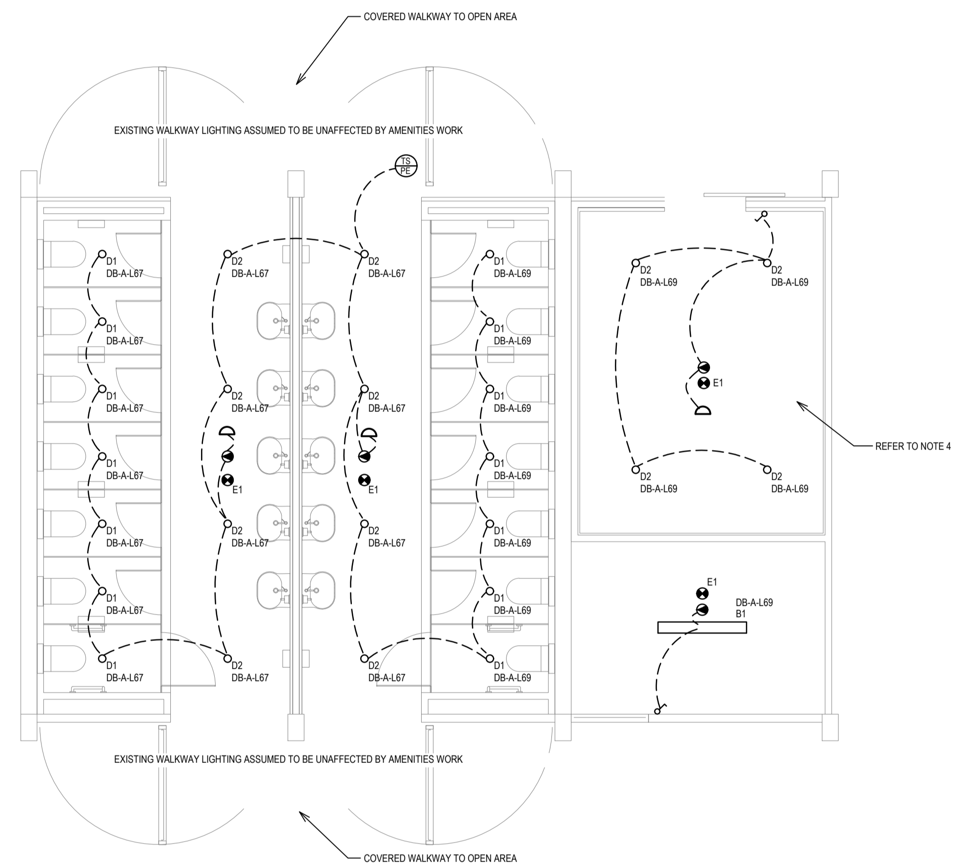
PROPOSED LIGHTING LAYOUT JUNIOR STUDENTS SCALE 1: 50
